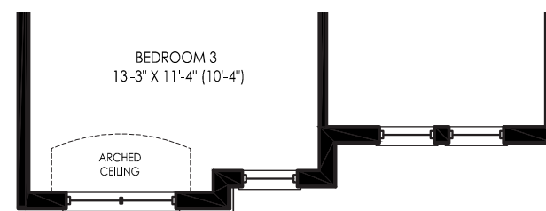
UPPER LEVEL
