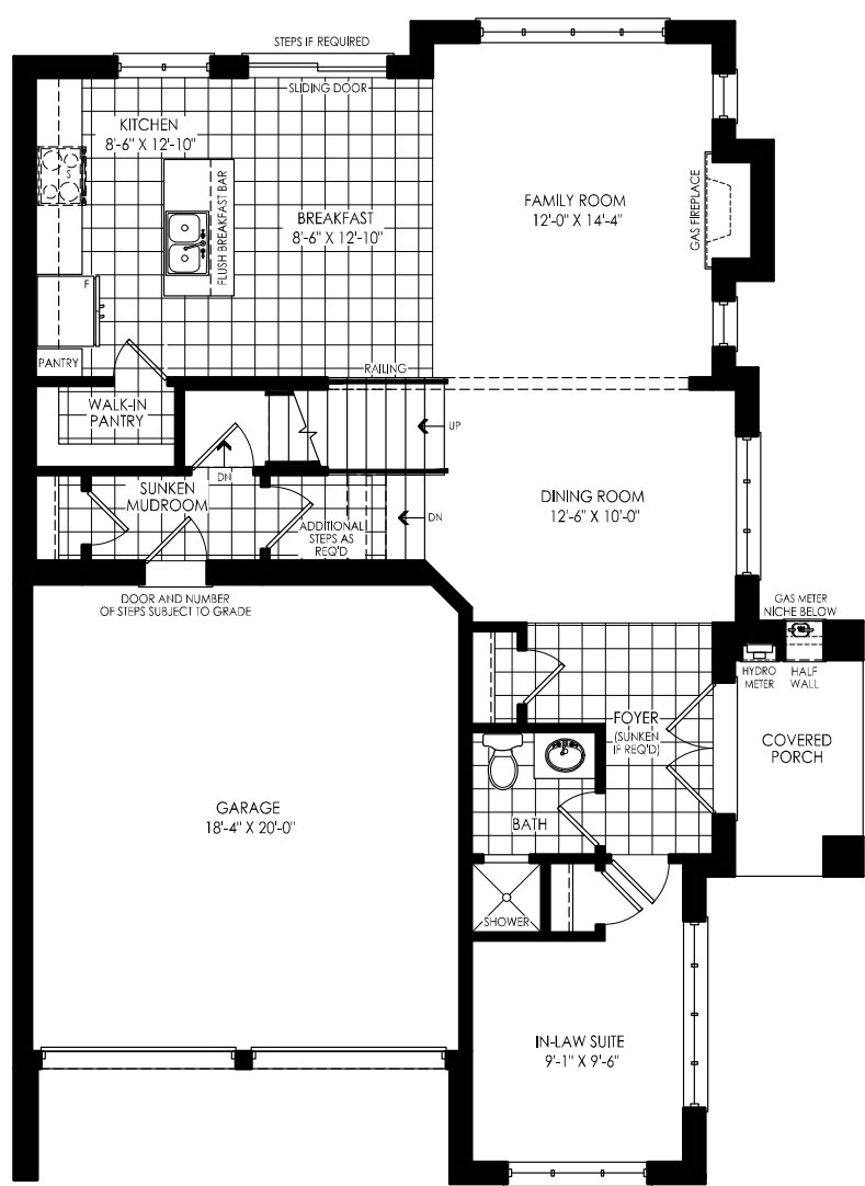
ELEV. A MAIN LEVEL W/ IN-LAW SUITE
