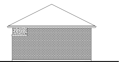
RIGHT SIDE ELEVATION - DOUBLE CAR GARAGE 'G-1' (STD.)
