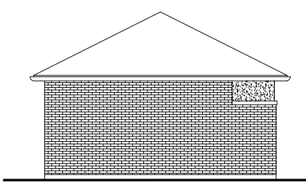
LEFT SIDE ELEVATION - DOUBLE CAR GARAGE 'G-1' & 'G-2' (STD.)
