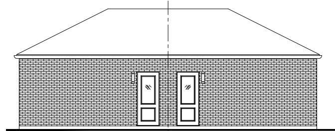
REAR ELEVATION - DOUBLE CAR GARAGE 'G-1' (STD.)
