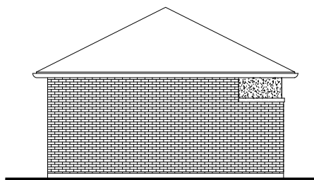
LEFT SIDE ELEVATION - DOUBLE CAR GARAGE 'G-1' & 'G-2' (STD.)
