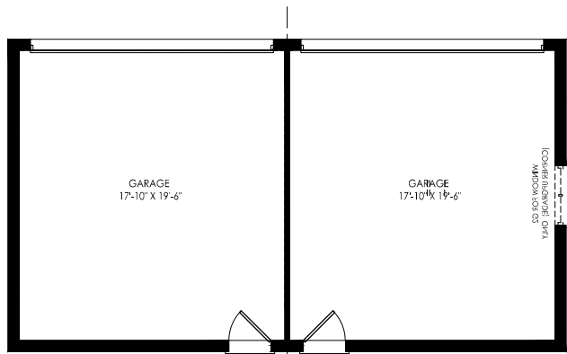
GROUND FLOOR PLAN 'G-1' & 'G-2'
