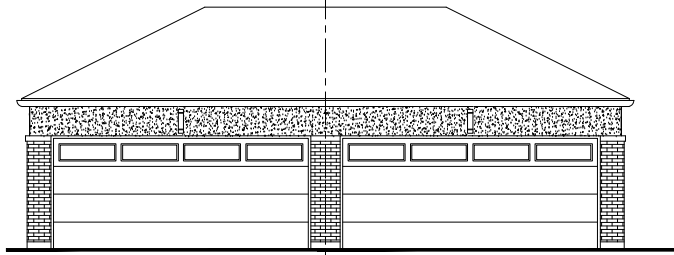
FRONT ELEVATION - DOUBLE CAR GARAGE 'G-1' & 'G-2' (STD. & CORNER UPGRADE)
