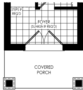
ELEV. B MAIN LEVEL
