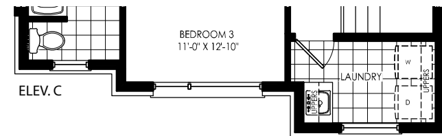
UPPER LEVEL
